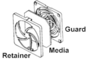
551147 Finger Guard
