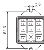
062.05 with relay
