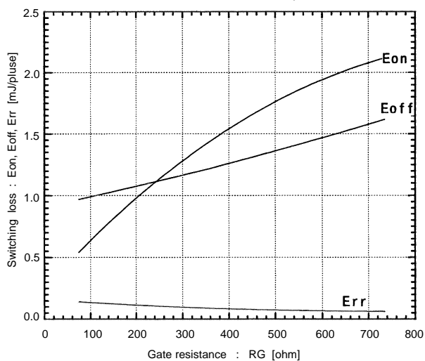
Switching loss vs. Gate resistance V_{cc}=300V, I_c=15A, V_{GE}=\pm 15V, T_j=125^\circ\text{C}
